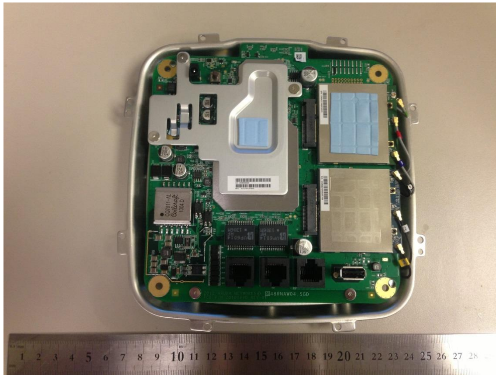
Photo 3 – Cover off View
