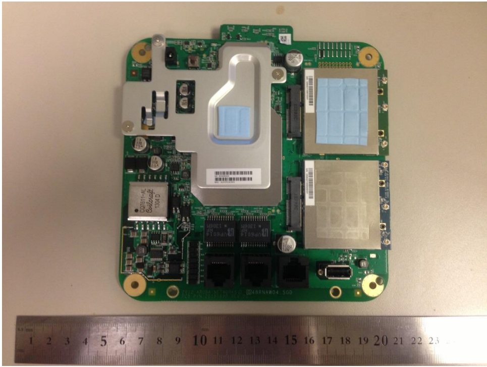
Photo 5 – Main Board Front View
